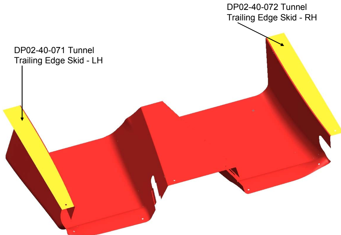
DP02 Tunnel Trailing Edge Skids
