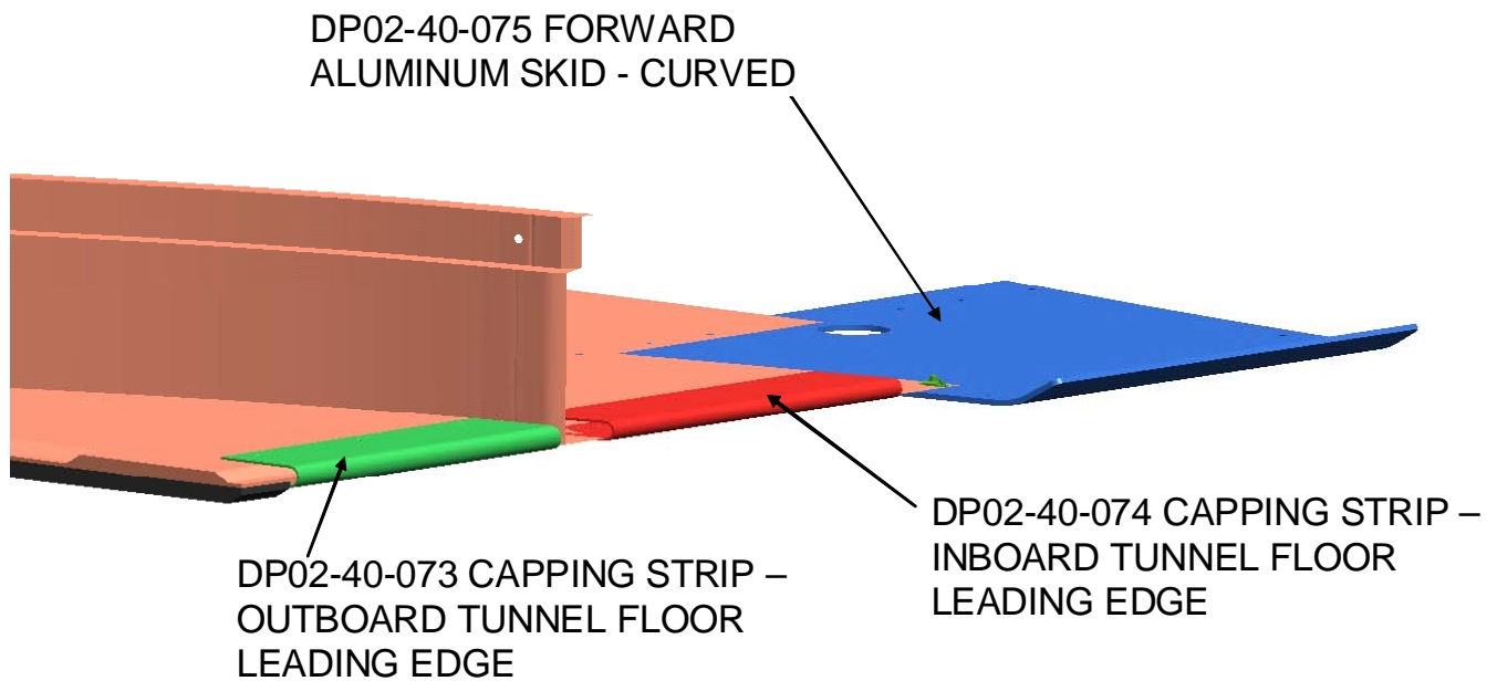
Figure 1: Optional skid components
