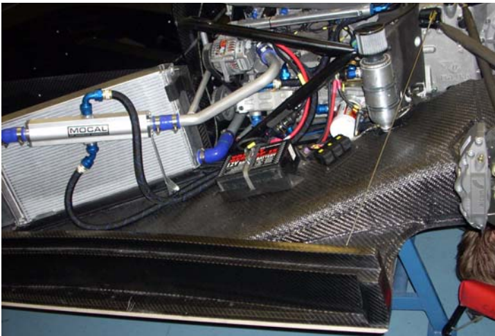
Engine Compartment & Rear Floor Stay LHS
